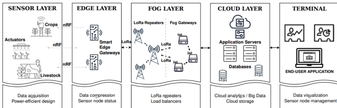
FIGURE 4. 5-layer Sensor-Edge-Fog-Cloud-Terminal SA [34]
